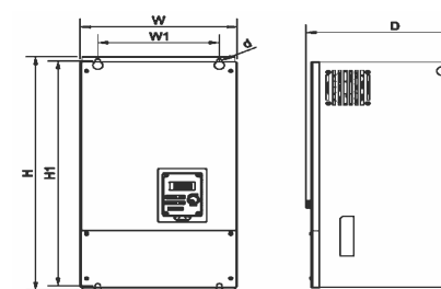
(图D)380V:40~75HP (IP20)
