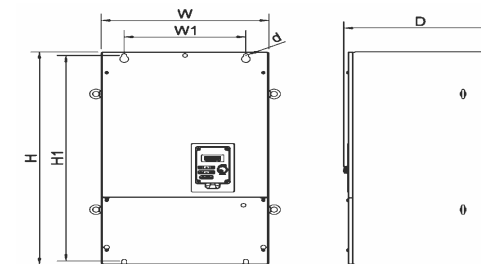
(图E)380V:100~335HP (IP00)
